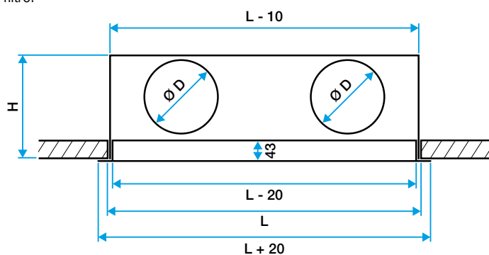
Plénium LINED
