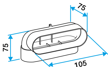
Coude vertical 90°
