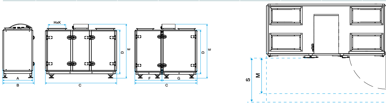
Dimensions VEX700T
